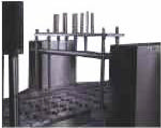
Automatic aluminum foil suction mechanism.
